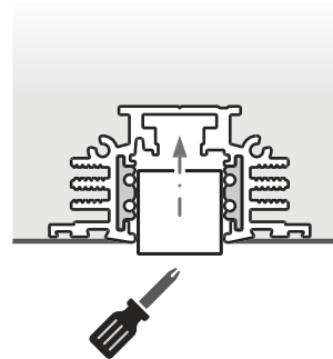
TRIMLESS ST3-EVO MECHANICAL FIXING
