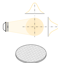
BEAM WIDTH LENSES 5031-0106 - 17° NARROW 5031-0037 - 25° NARROW FLOOD 5031-0038 - 36° FLOOD 5031-0039 - 60° WIDE FLOOD
